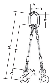
AN2G AT Braca a due tratti con campanella, radance e ganci Two legs sling with master link, thimble and hoist hook I min=33xØ
