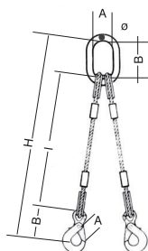
AN2G AT Braca a due tratti con campanella, radance e ganci Two legs sling with master link, thimble and hoist hook I min=33xØ
