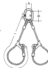
AN2GSL AT Braca a due tratti con campanella, radance e ganci Two legs sling with master link, thimble and hoist hook I min=33xØ
